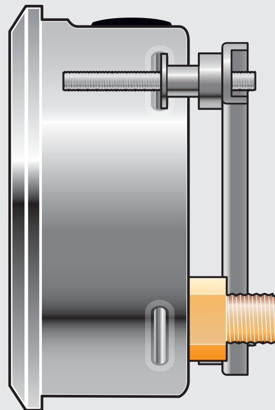
4" Stainless Steel Case Gauge
